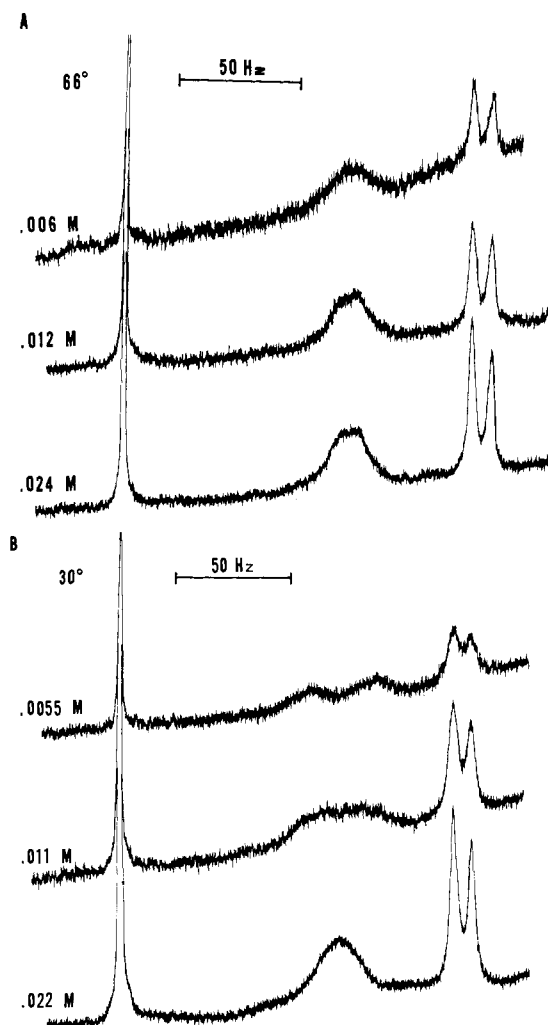
Figure 5. (A) ^1\text{H} NMR spectra (100 MHz) of phenyl region for \text{In}(p\text{-}i\text{-PrTPP})\text{Cl} in 1,1,2,2-tetrachloroethane at various concentrations. 34 (B) ^1\text{H} NMR spectra (100 MHz) of \text{In}(p\text{-}i\text{-PrTPP})\text{Cl} in the presence of n\text{-Bu}_4\text{NCl} at 30°. The ratio of n\text{-Bu}_4\text{NCl} to \text{In}(p\text{-}i\text{-PrTPP})\text{Cl} is constant at 0.23. The concentration of \text{In}(p\text{-}i\text{-PrTPP})\text{Cl} is given to the left of each spectrum.
