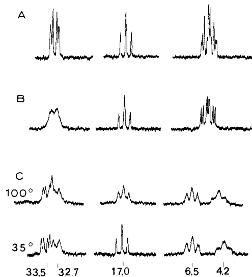
Figure 2. ^{19}\text{F} NMR spectra (56 MHz) of 1,1,2,2-tetrachloroethane solutions of: A, \text{H}_2(\text{F}_5\text{TPP}) at 30^\circ ; B, \text{In}(\text{F}_5\text{TPP})\text{Cl} in the presence of excess n\text{-Bu}_4\text{NCl} at 35^\circ ; C, \text{In}(\text{F}_5\text{TPP})\text{Cl} at 35^\circ and 100^\circ . Chemical shifts are in parts per million downfield of external neat \text{C}_6\text{F}_6 : o -F, 33.5, 32.7; p -F, 17.0; m -F, 6.5, 4.2.
